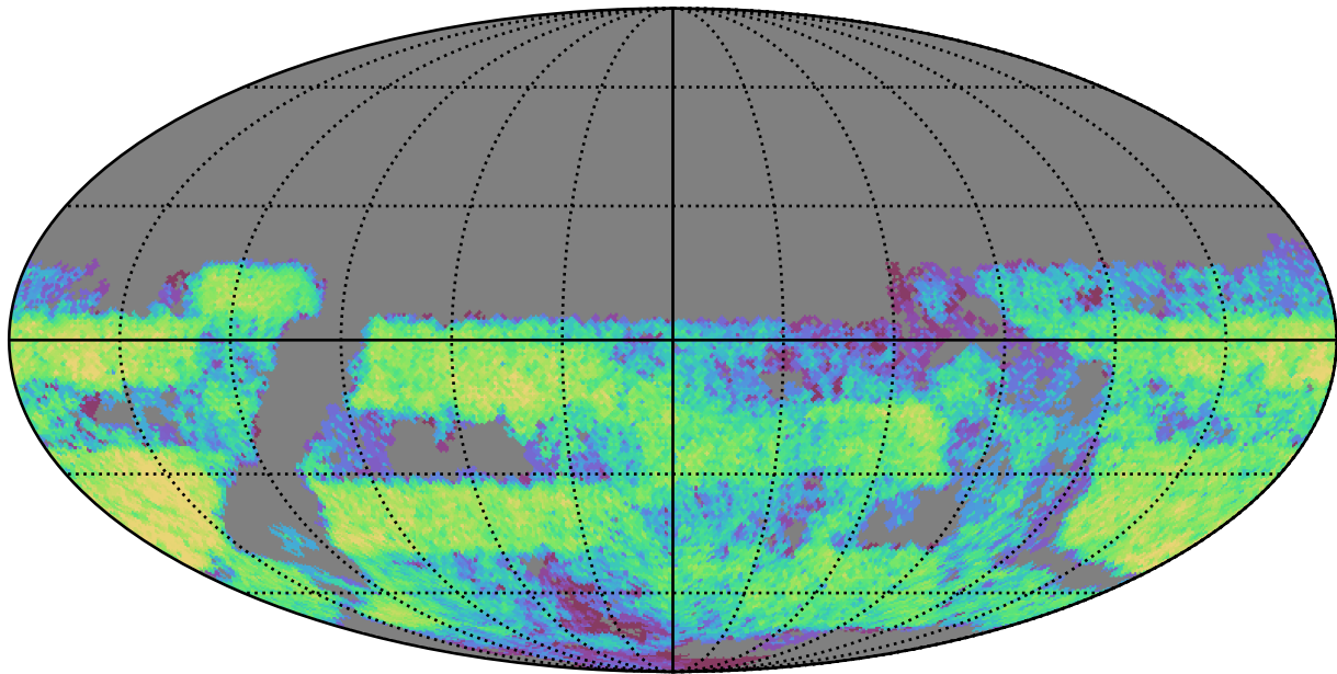
too_100_4v3.4_10yrs Yr 3-4 u band: CoaddM5
