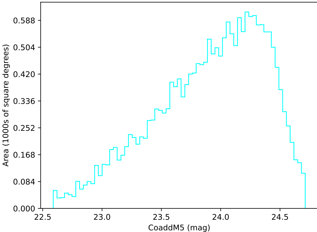
too_100_4v3.4_10yrs Yr 3-4 u band: CoaddM5
