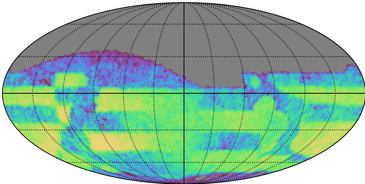
too_100_4v3.4_10yrs Yr 3-4 r band: CoaddM5
