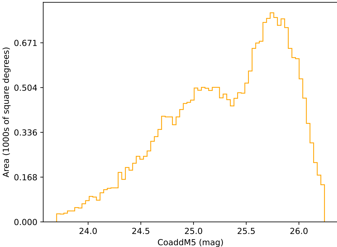
too_100_4v3.4_10yrs Yr 3-4 r band: CoaddM5
