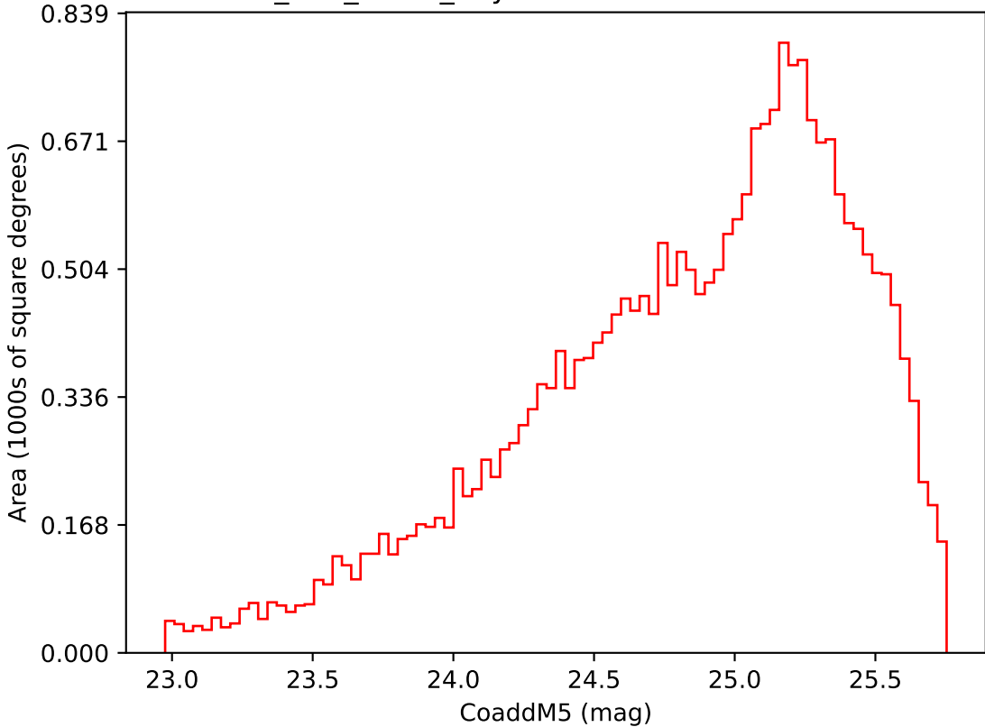
too_100_4v3.4_10yrs Yr 3-4 i band: CoaddM5
