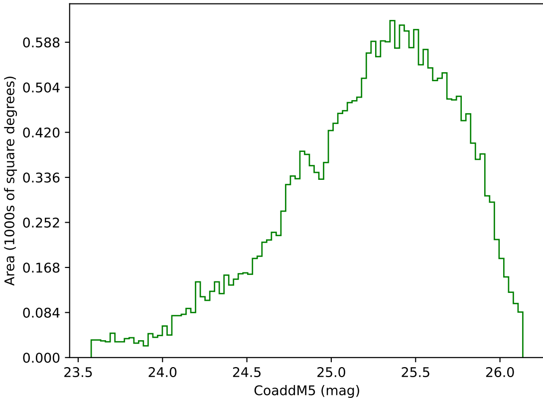
too_100_4v3.4_10yrs Yr 3-4 g band: CoaddM5
