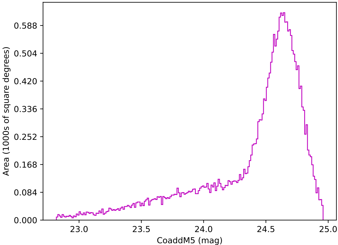
too_100_4v3.4_10yrs Yr 1 z band: CoaddM5
