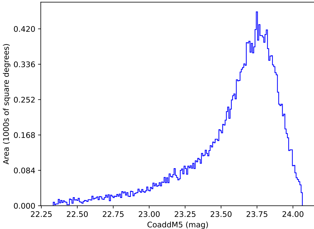
too_100_4v3.4_10yrs Yr 1 y band: CoaddM5
