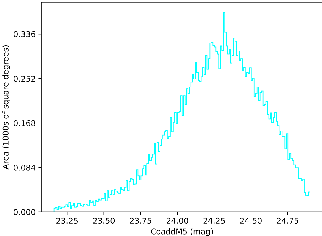
too_100_4v3.4_10yrs Yr 1 u band: CoaddM5
