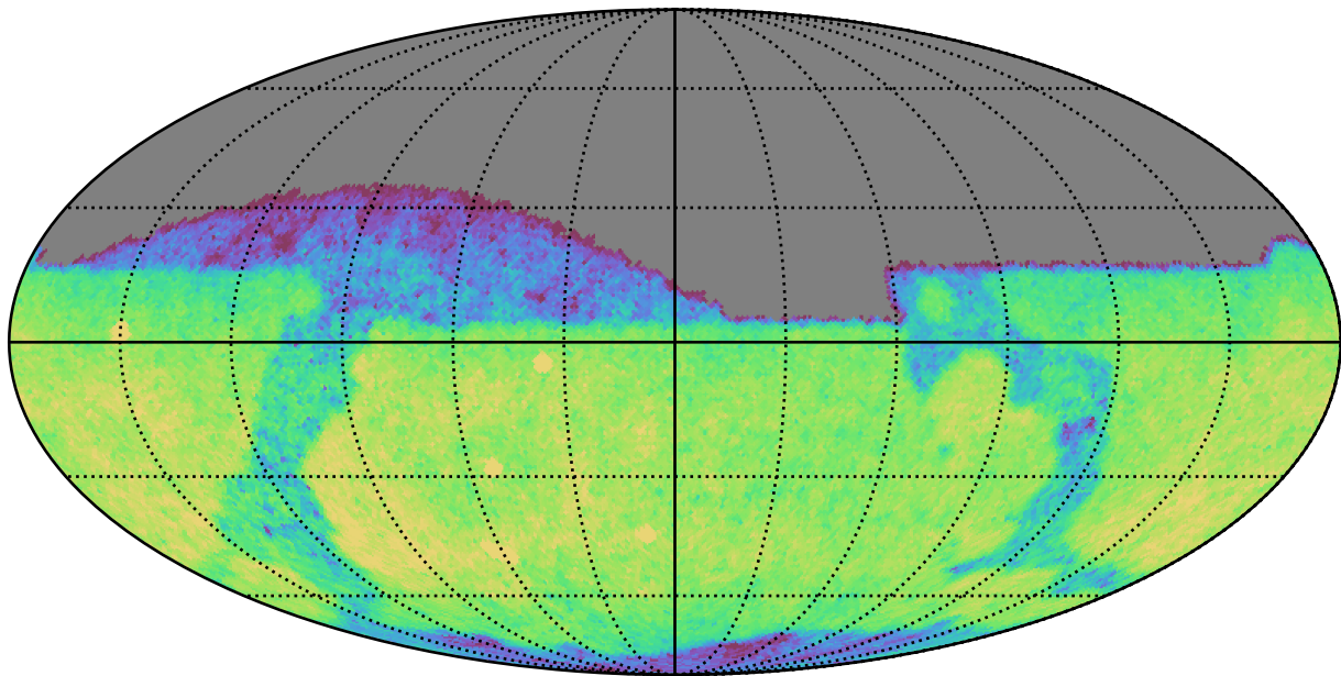
too_100_4v3.4_10yrs Yr 1 r band: CoaddM5
