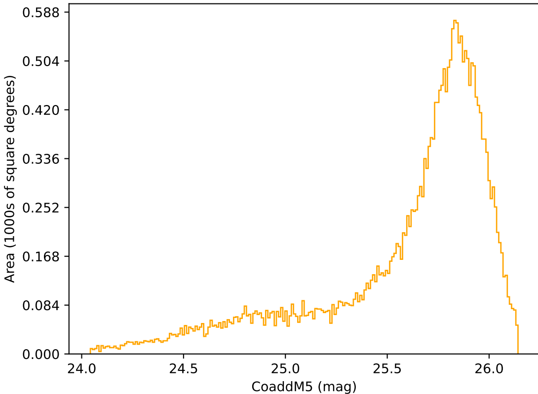
too_100_4v3.4_10yrs Yr 1 r band: CoaddM5
