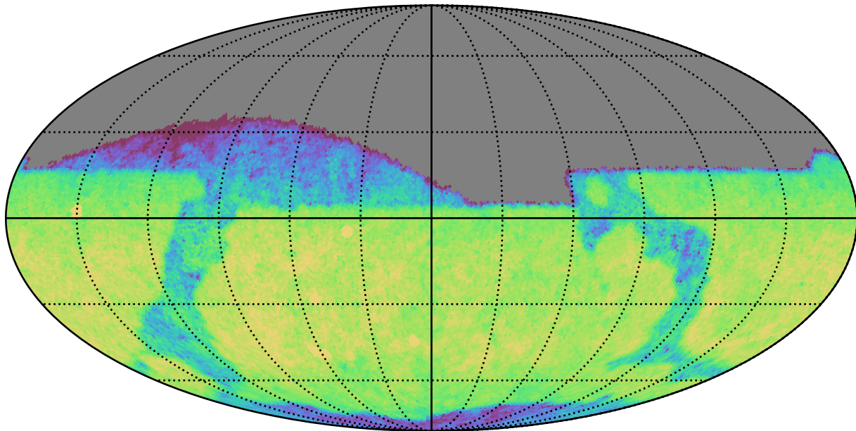
too_100_4v3.4_10yrs Yr 1 i band: CoaddM5
