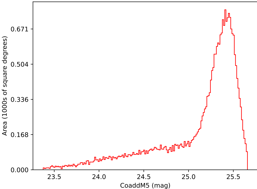
too_100_4v3.4_10yrs Yr 1 i band: CoaddM5
