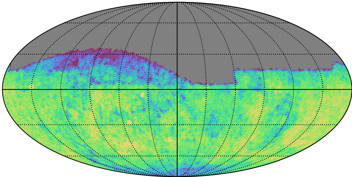
too_100_4v3.4_10yrs Yr 1 g band: CoaddM5
