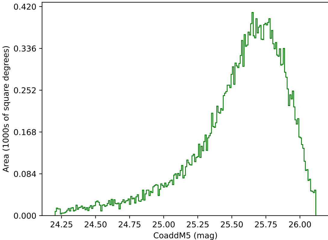
too_100_4v3.4_10yrs Yr 1 g band: CoaddM5
