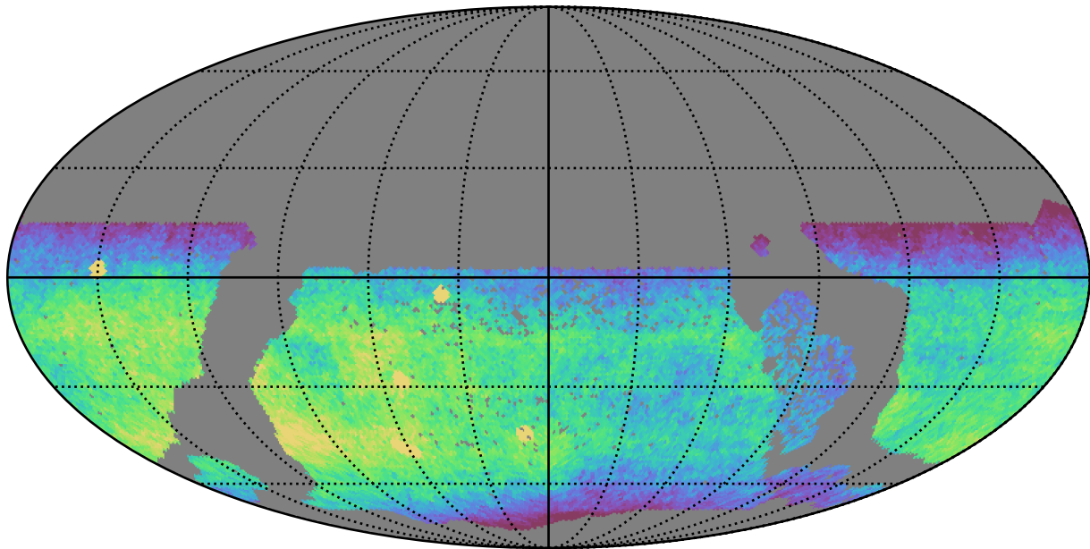
too_100_4v3.4_10yrs WFD z band: CoaddM5
