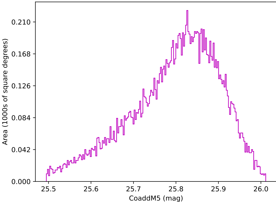
too_100_4v3.4_10yrs WFD z band: CoaddM5
