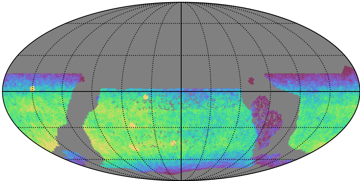
too_100_4v3.4_10yrs WFD y band: CoaddM5
