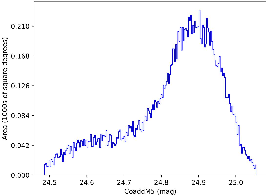
too_100_4v3.4_10yrs WFD y band: CoaddM5
