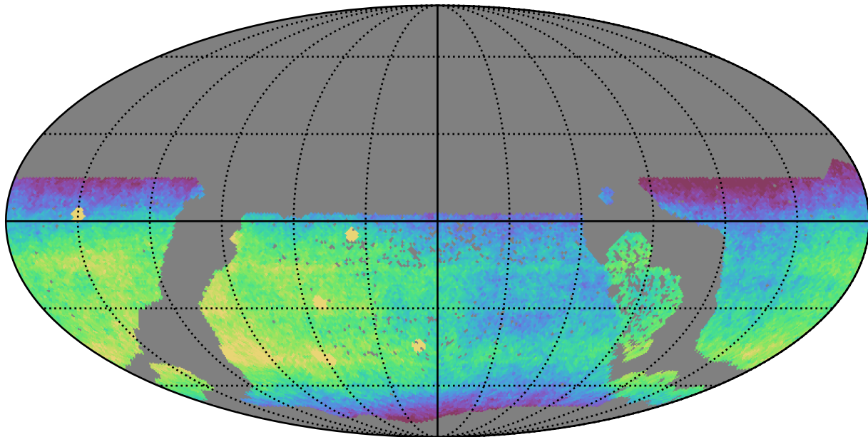
too_100_4v3.4_10yrs WFD r band: CoaddM5
