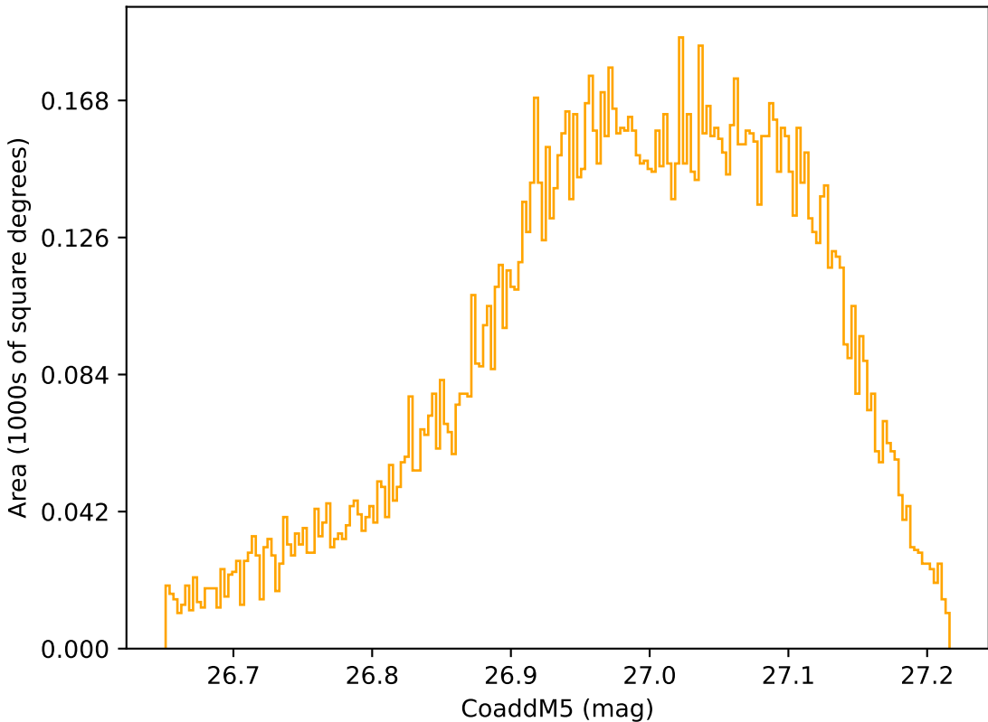
too_100_4v3.4_10yrs WFD r band: CoaddM5
