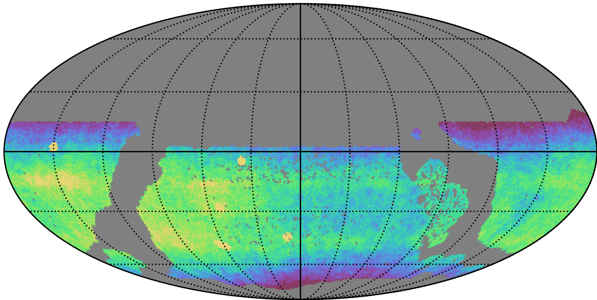
too_100_4v3.4_10yrs WFD i band: CoaddM5
