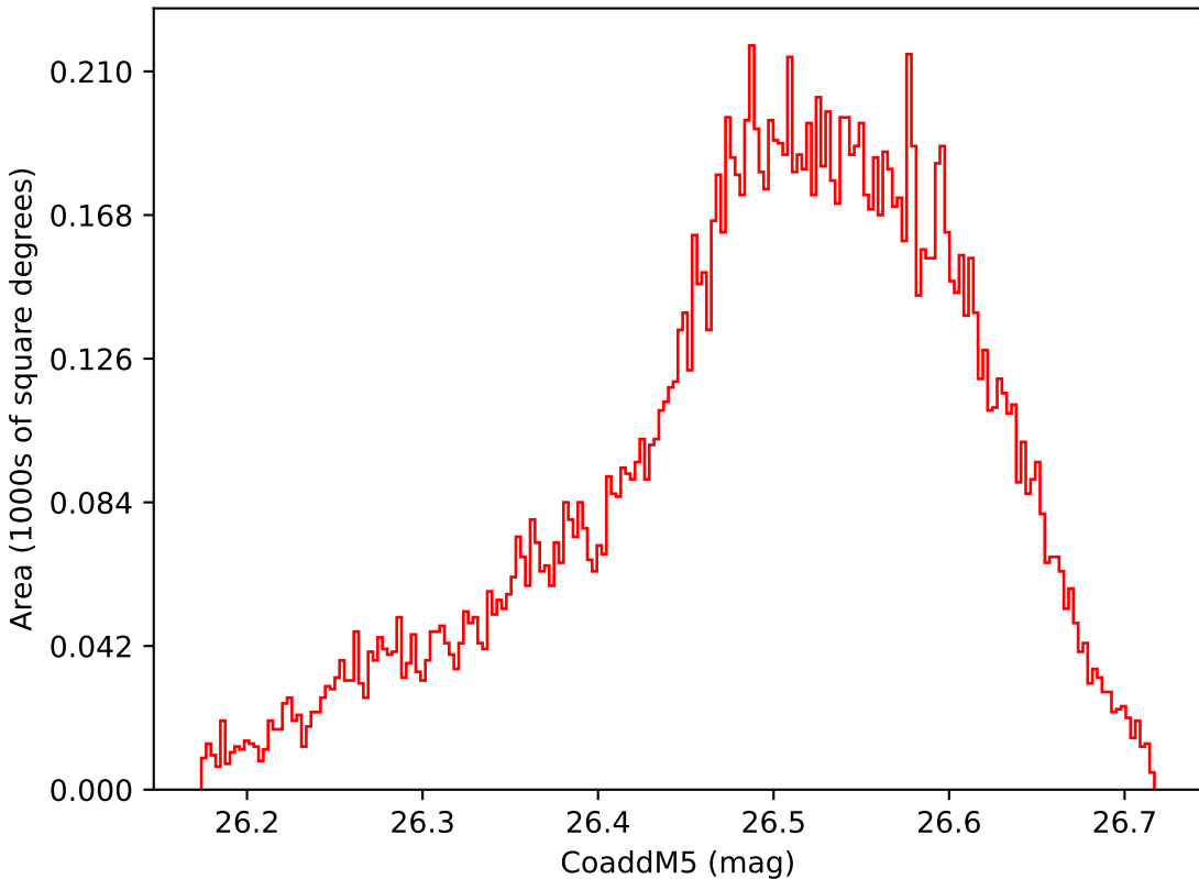
too_100_4v3.4_10yrs WFD i band: CoaddM5
