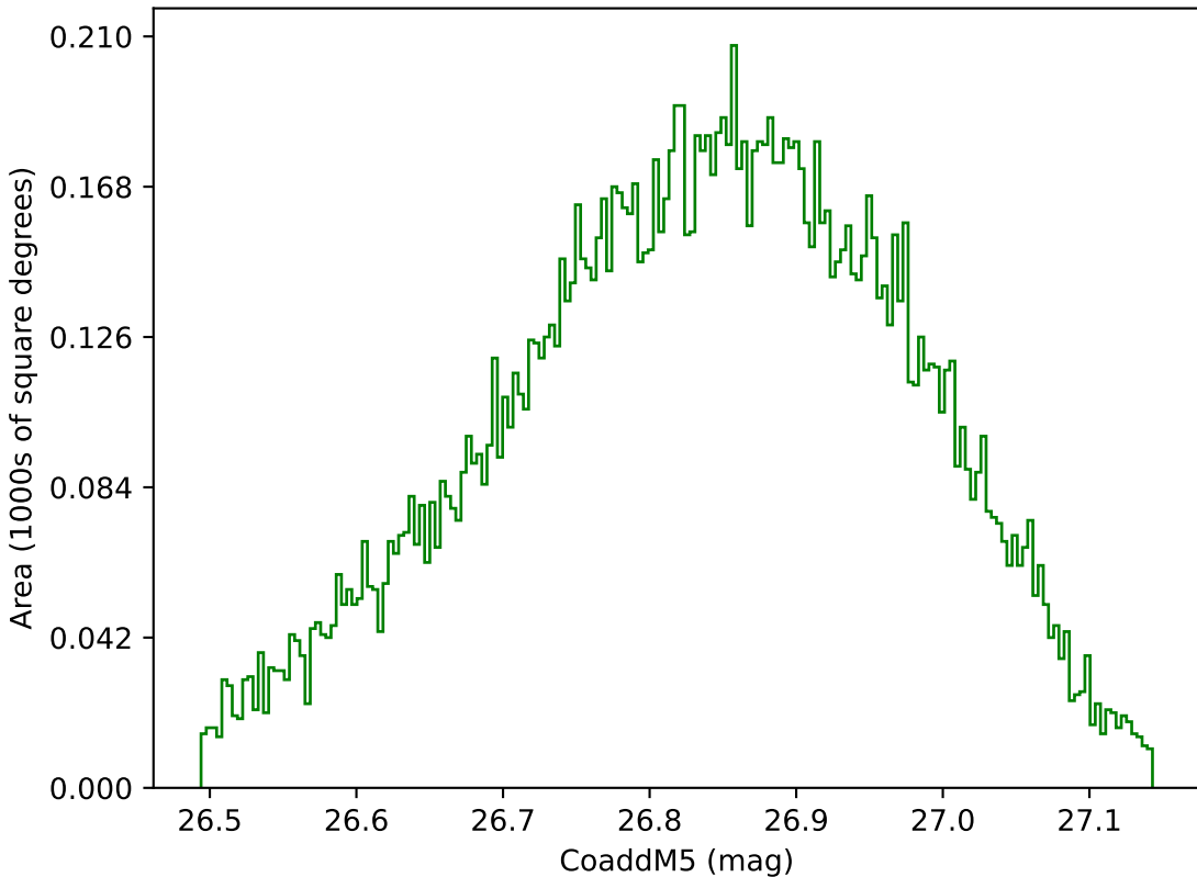
too_100_4v3.4_10yrs WFD g band: CoaddM5
