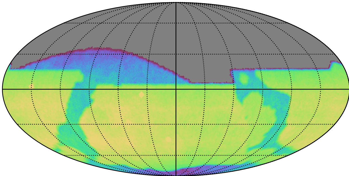
too_100_4v3.4_10yrs All sky z band: CoaddM5
