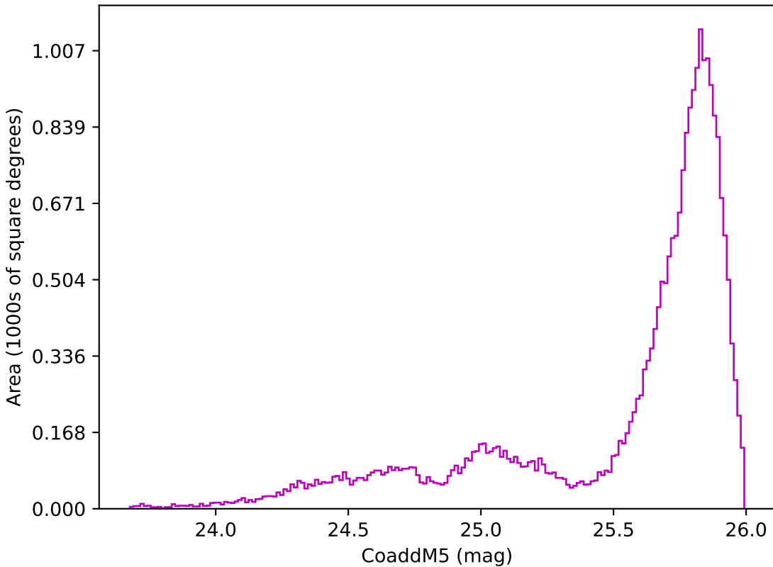
too_100_4v3.4_10yrs All sky z band: CoaddM5
