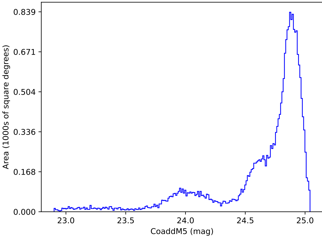
too_100_4v3.4_10yrs All sky y band: CoaddM5
