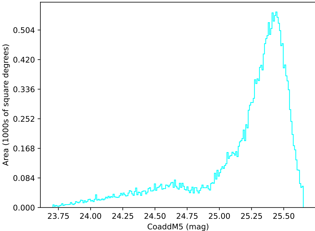
too_100_4v3.4_10yrs All sky u band: CoaddM5
