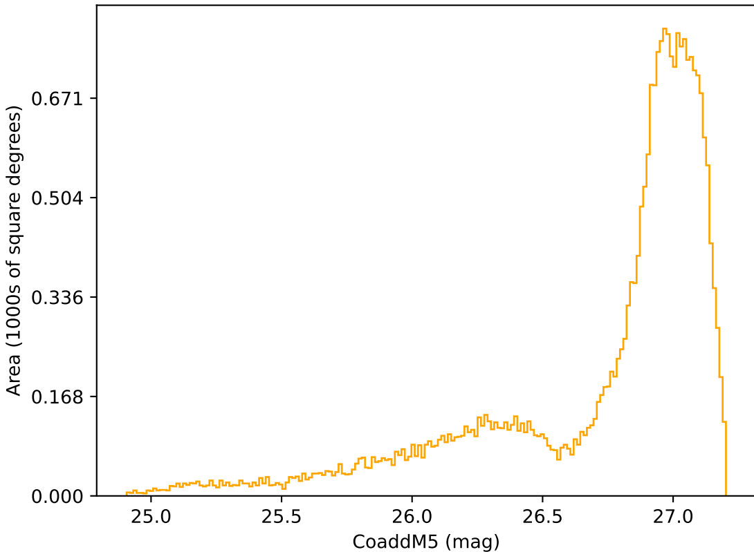
too_100_4v3.4_10yrs All sky r band: CoaddM5
