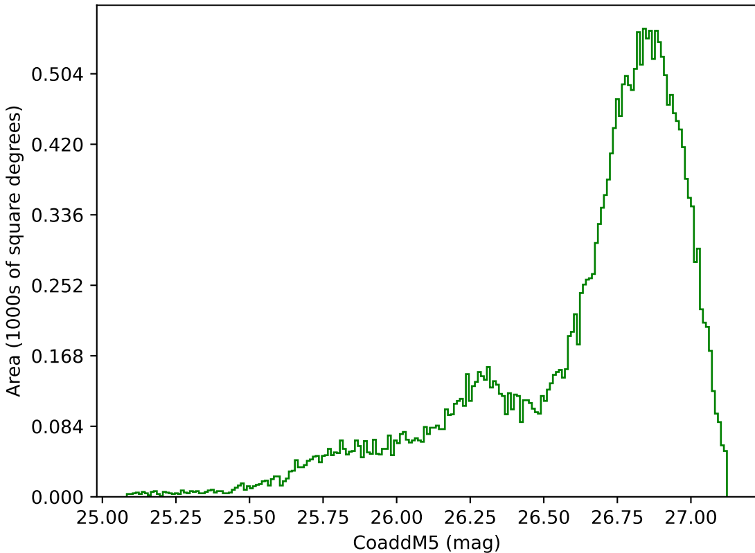
too_100_4v3.4_10yrs All sky g band: CoaddM5
