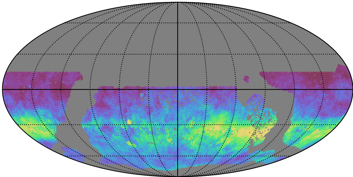
too_100_4v3.4_10yrs WFD z band: AngleRms rotSkyPos
