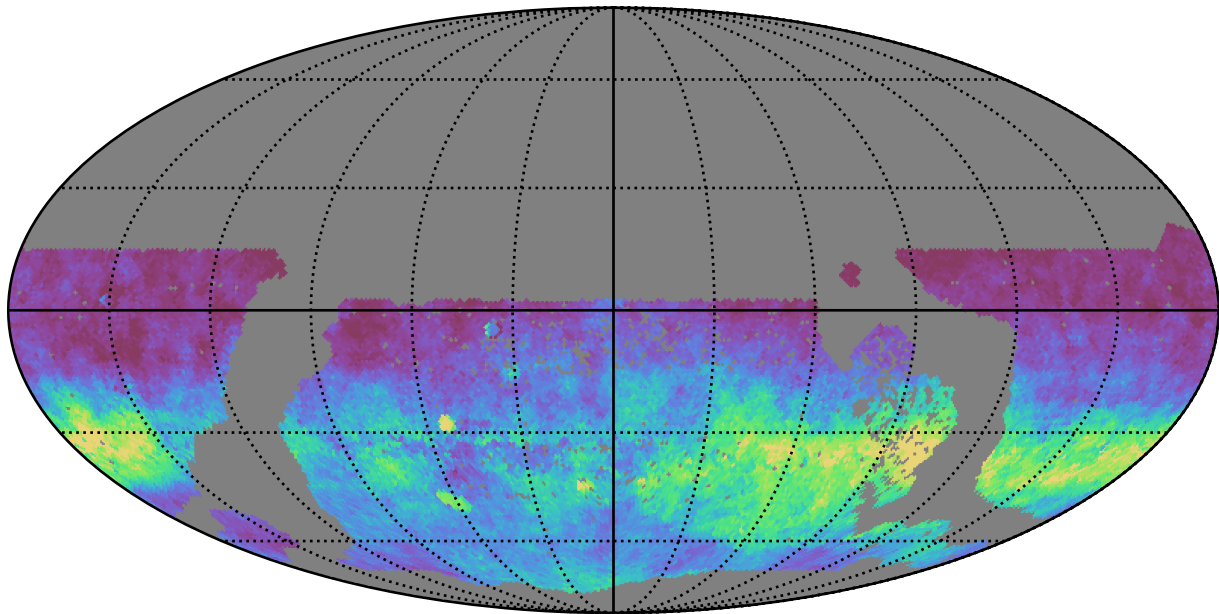
too_100_4v3.4_10yrs WFD i band: AngleRms rotSkyPos
