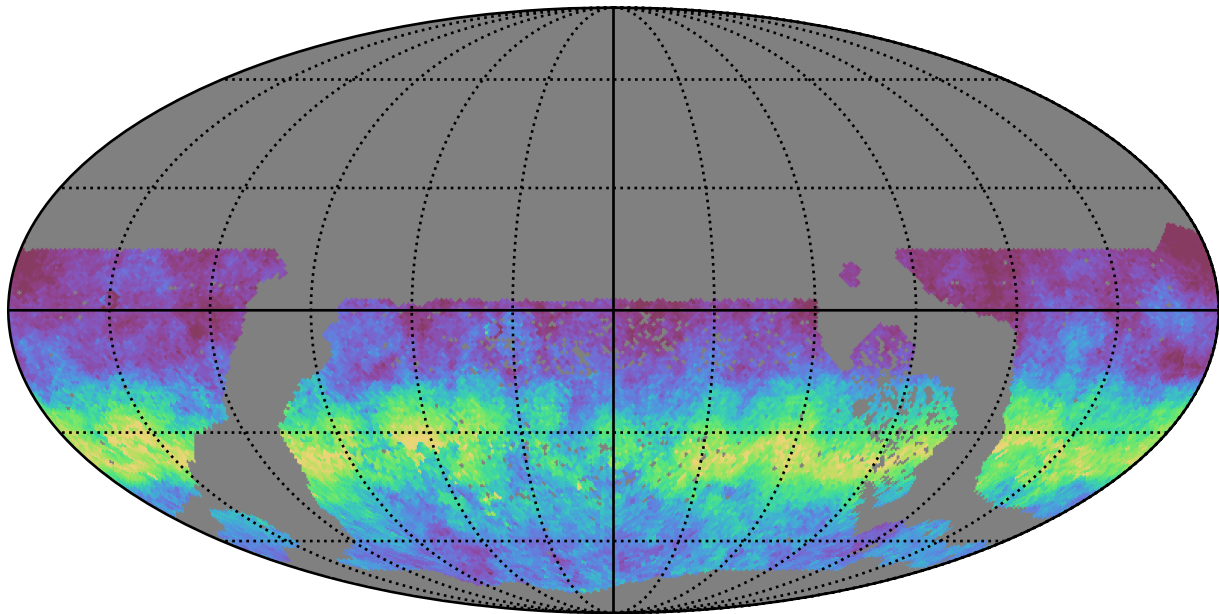
too_100_4v3.4_10yrs WFD g band: AngleRms rotSkyPos
