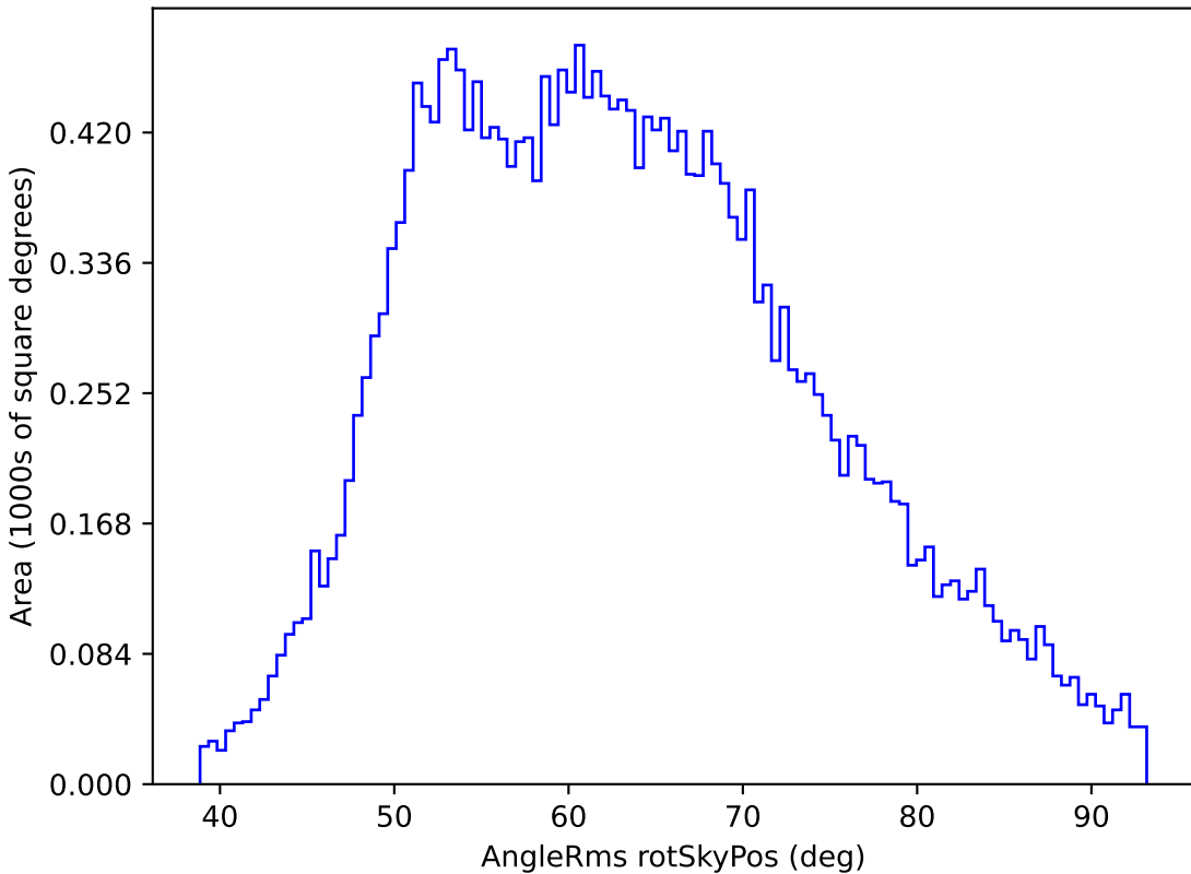
too_100_4v3.4_10yrs All sky z band: AngleRms rotSkyPos
