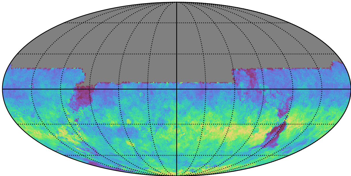
too_100_4v3.4_10yrs All sky u band: AngleRms rotSkyPos
