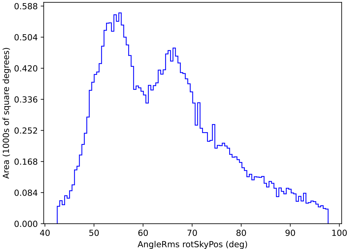
too_100_4v3.4_10yrs All sky r band: AngleRms rotSkyPos
