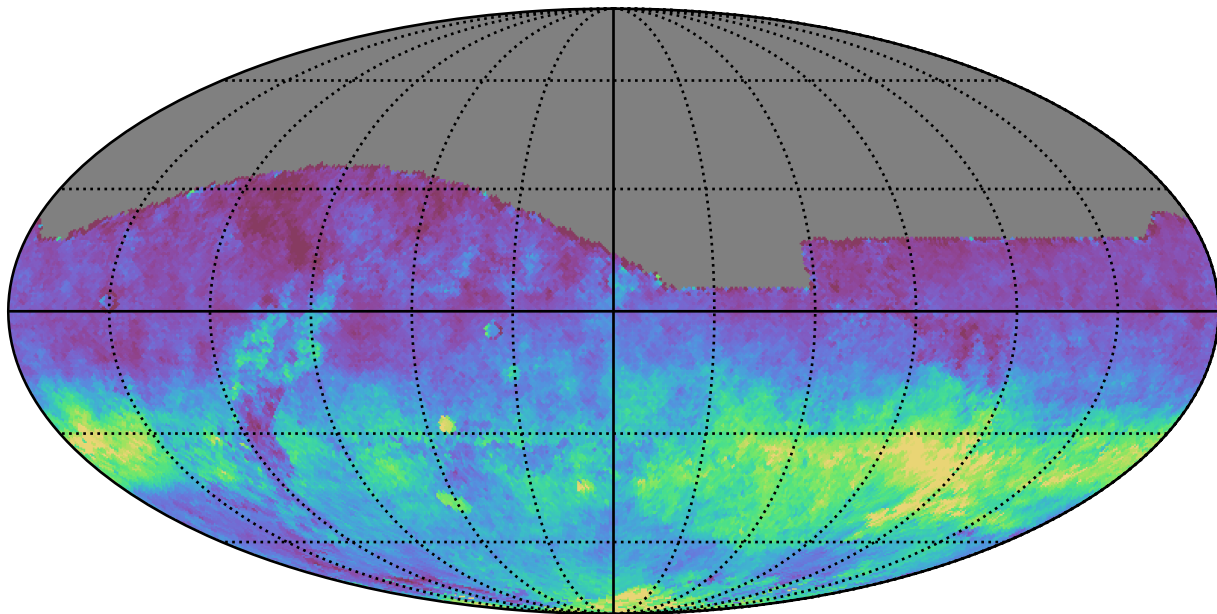
too_100_4v3.4_10yrs All sky i band: AngleRms rotSkyPos
