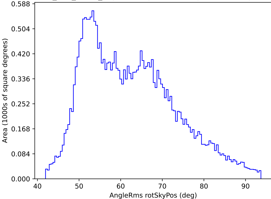
too_100_4v3.4_10yrs All sky i band: AngleRms rotSkyPos
