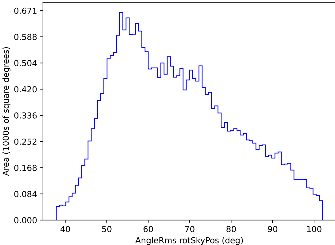
too_100_4v3.4_10yrs All sky g band: AngleRms rotSkyPos
