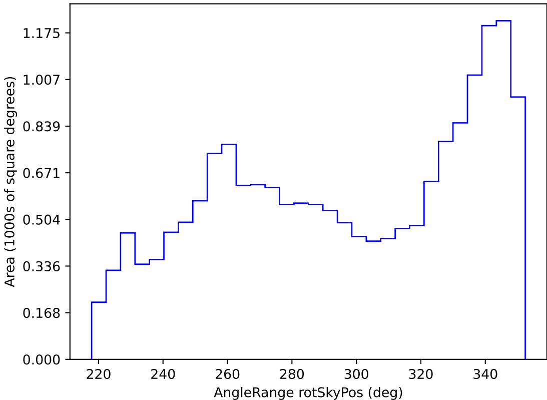
too_100_4v3.4_10yrs WFD all bands: AngleRange rotSkyPos
