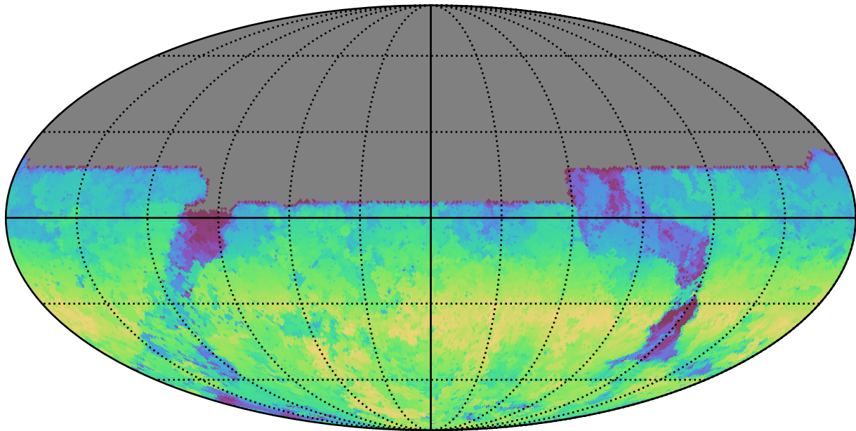
too_100_4v3.4_10yrs All sky u band: AngleRange rotSkyPos
