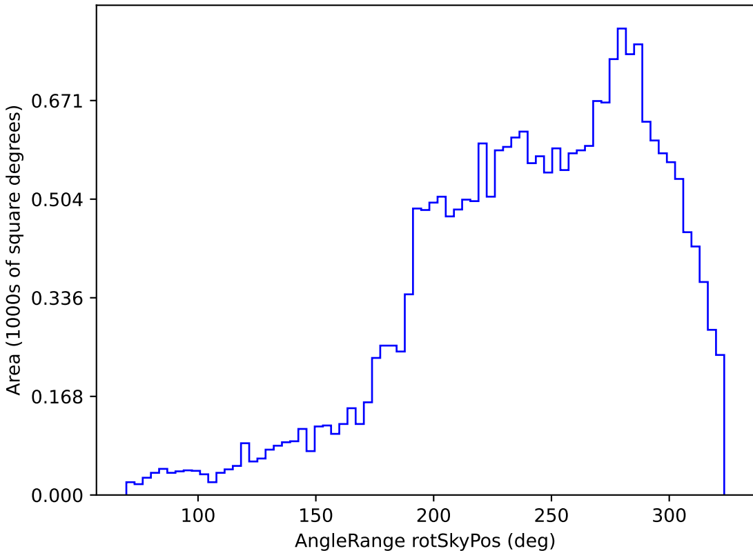
too_100_4v3.4_10yrs All sky u band: AngleRange rotSkyPos
