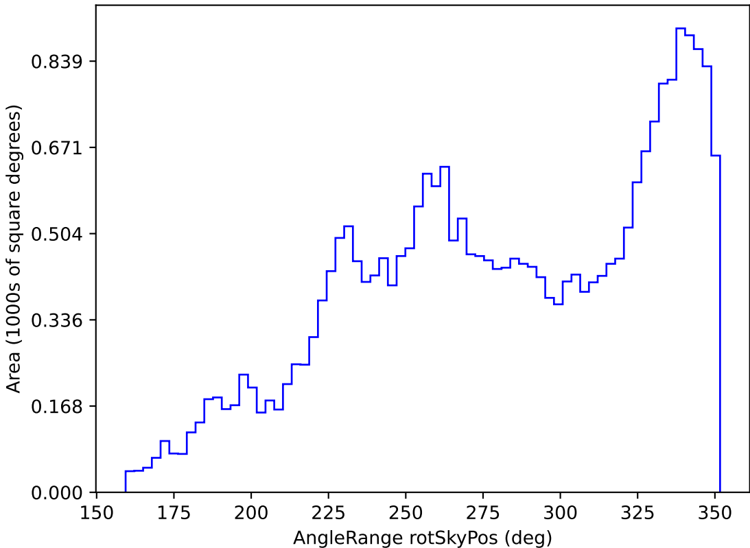
too_100_4v3.4_10yrs All sky all bands: AngleRange rotSkyPos
