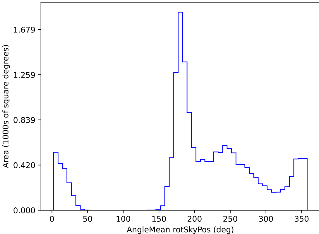
too_100_4v3.4_10yrs WFD z band: AngleMean rotSkyPos
