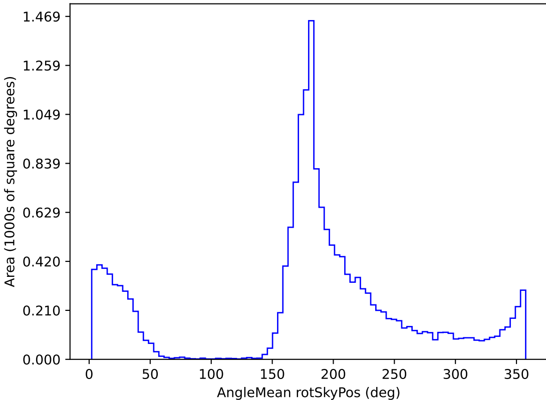
too_100_4v3.4_10yrs WFD g band: AngleMean rotSkyPos
