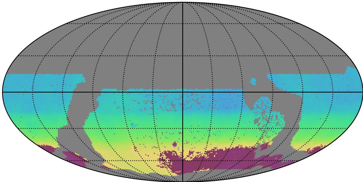
too_100_4v3.4_10yrs WFD all bands: AngleMean rotSkyPos
