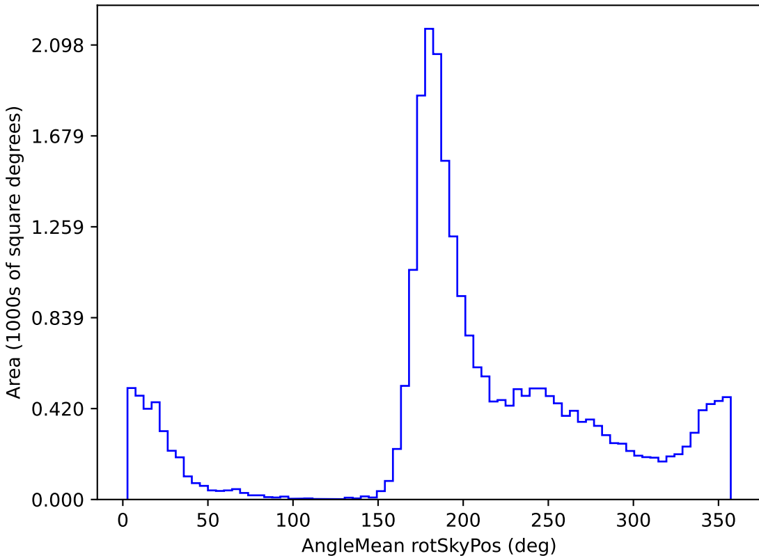
too_100_4v3.4_10yrs All sky z band: AngleMean rotSkyPos
