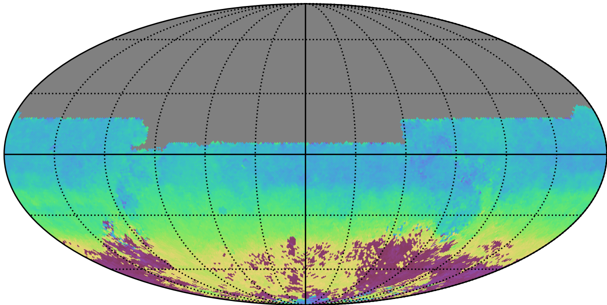
too_100_4v3.4_10yrs All sky u band: AngleMean rotSkyPos
