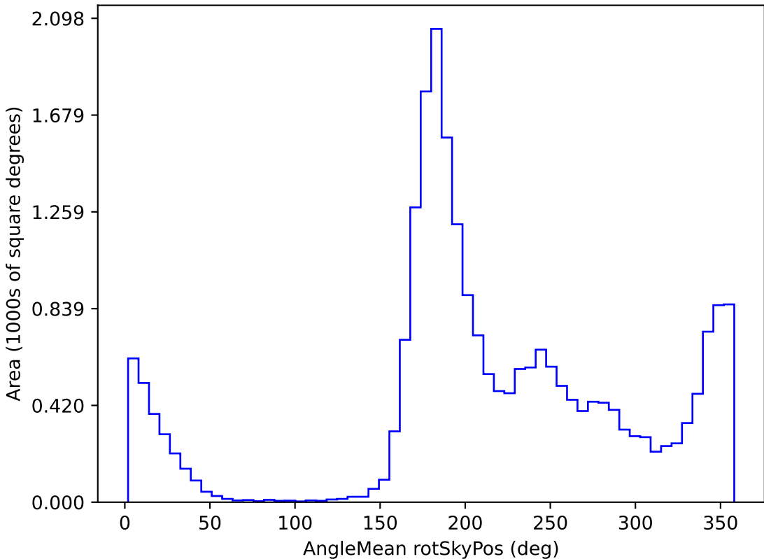
too_100_4v3.4_10yrs All sky u band: AngleMean rotSkyPos
