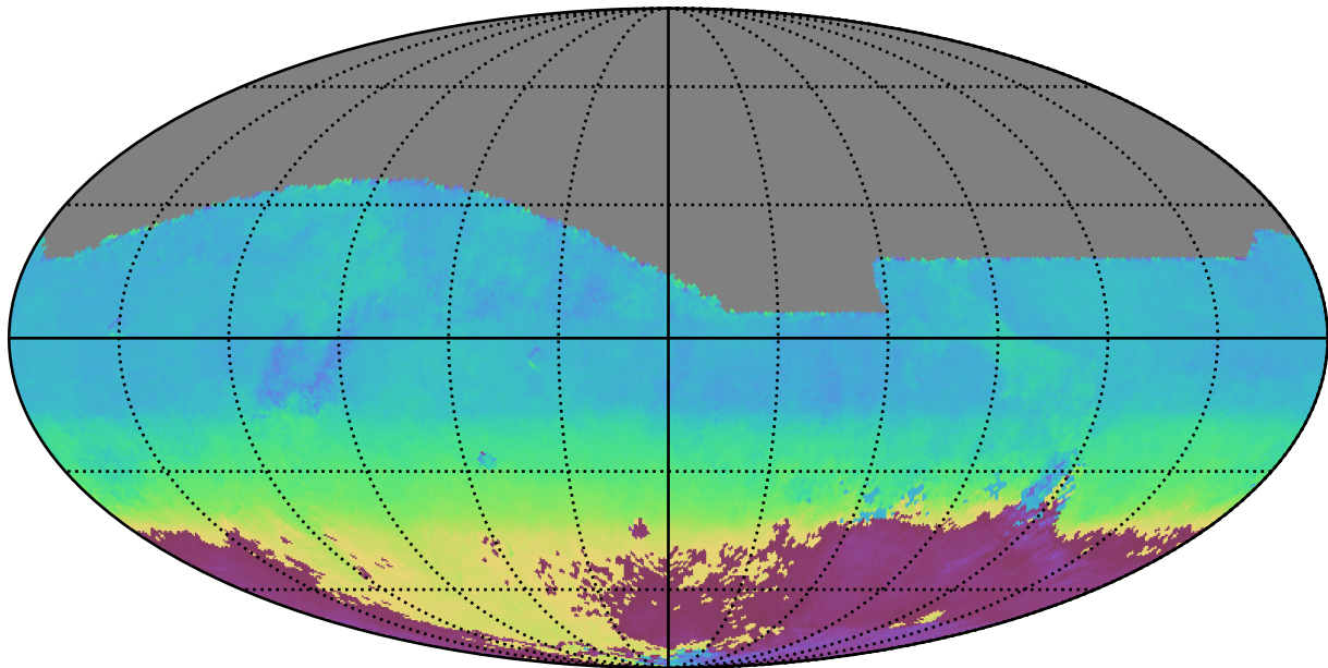
too_100_4v3.4_10yrs All sky r band: AngleMean rotSkyPos
